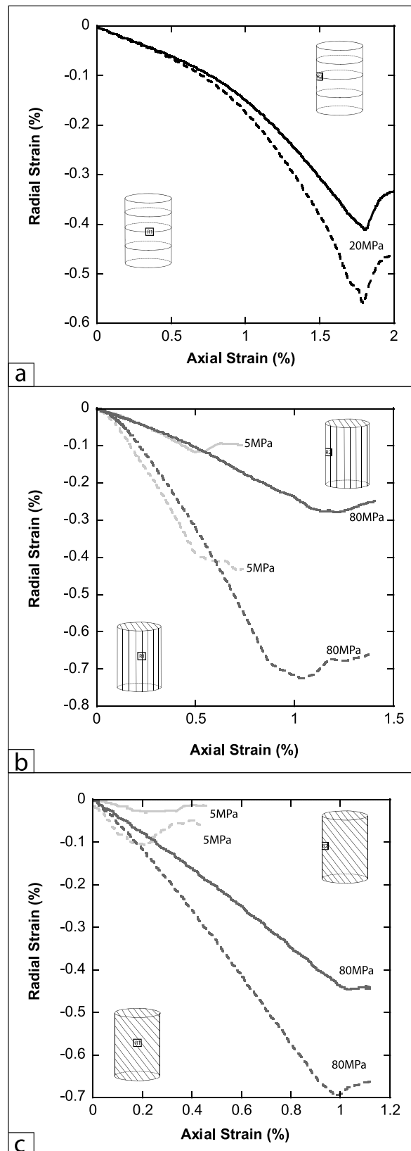
Figure 6. Radial strain (%) as a function of axial strain (at the locations R1 (dashed lines) and R2 (solid lines)) for three bedding orientations: (a) for \phi = 90^\circ and confining pressure 20 MPa, (b) for \phi = 0^\circ and confining pressures 5 and 80 MPa, and (c) for \phi = 45^\circ and confining pressures 5 and 80 MPa.
