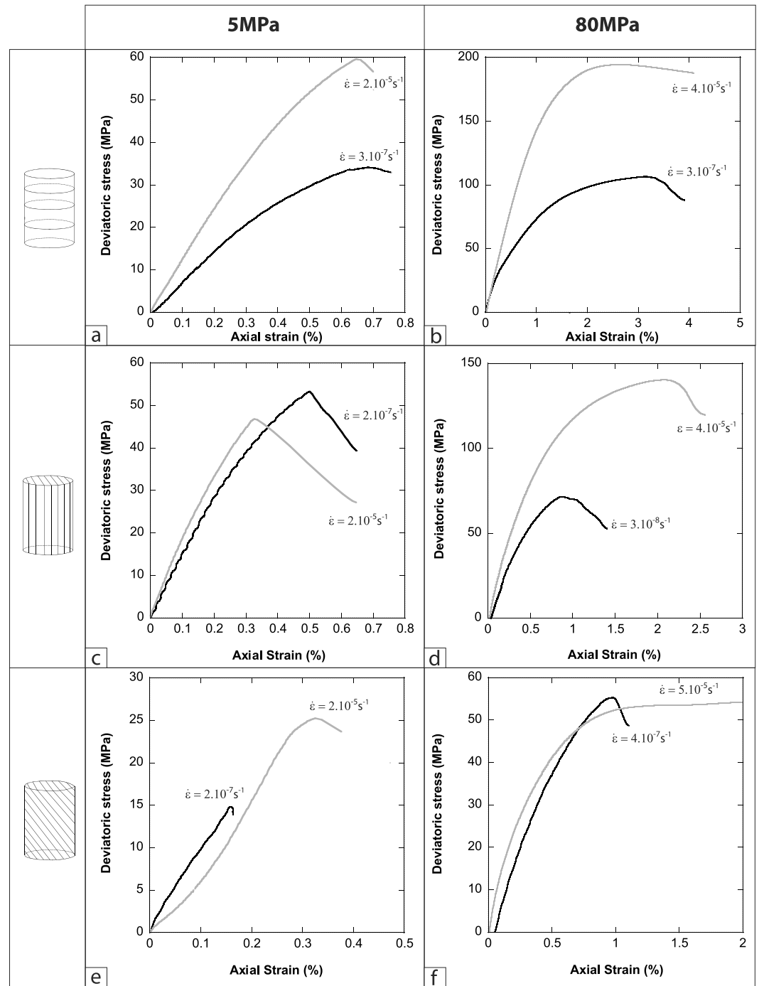
Figure 8. Deviatoric stress ( \sigma_1 - \sigma_3 , MPa) as a function of axial strain (%) for confining pressures of (a, c, and e) 5 MPa and (b, d, and f) 80 MPa and for three bedding orientations \phi = 90^\circ (Figures 8a and 8b), \phi = 0^\circ (Figures 8c and 8d), and \phi = 45^\circ (Figures 8e and 8f), high strain rate (grey curve) and low strain rate (black curve).
