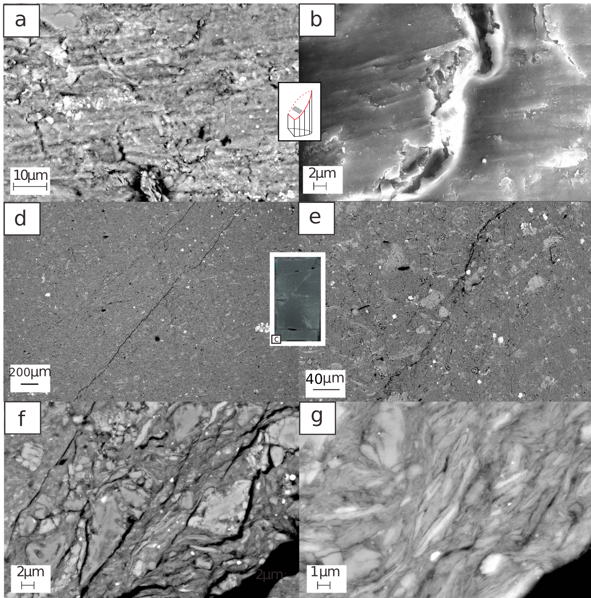
Figure 11. (a and b) Scanning electron micrograph of the fracture plane of sample deformed parallel to bedding ( \phi = 0^\circ ) and 80 MPa confining pressure at a strain rate of 3 \times 10^{-5} \text{ s}^{-1} . (c–g) Fracture on a sample deformed perpendicular to bedding ( \phi = 90^\circ ) at 160 MPa confining pressure.
