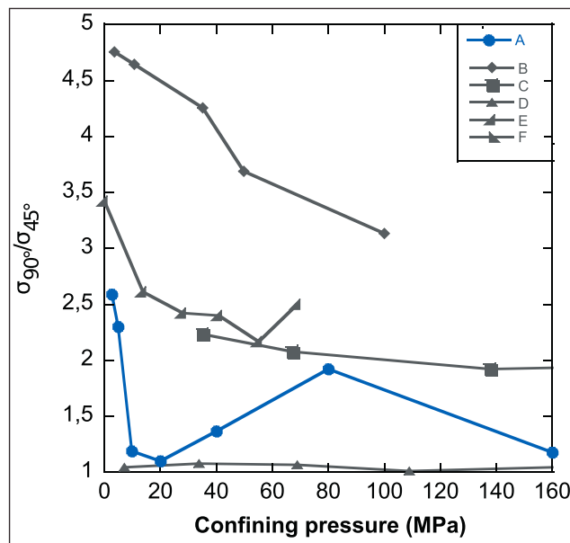
Figure 13. Ratios of peak deviatoric stress for the orientation 90° to peak deviatoric stress for the orientation 45° with A: our data at slow strain rate, B: Martinsburg slate from Donath and Parker [1964], C: Austin slate from McLamore and Gray [1967], D: Green River shale from McLamore and Gray [1967], E: Blue Penrhyn slate from Attewell and Sandford [1974], and F: limestone from Horino and Ellickson [1970].
