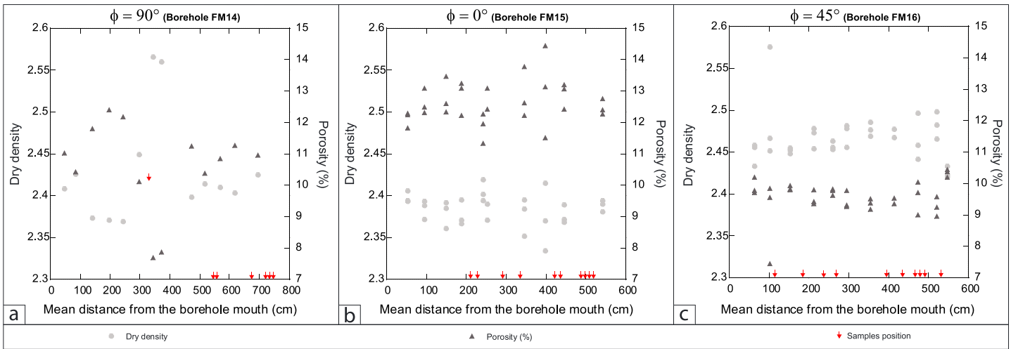
Figure 2. Dry density (light grey dots) and porosity (%), measured in the field, as a function of the distance from the borehole mouth (cm), for each bedding orientation. The red squares represent the position where the samples used for mechanical tests were taken.
