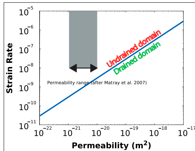
Figure 15. Critical strain rate line as a function of permeability ( \text{m}^2 ) from Duda and Renner [2012] equation. The grey shaded area represents the domain in which the experiments were performed here.
