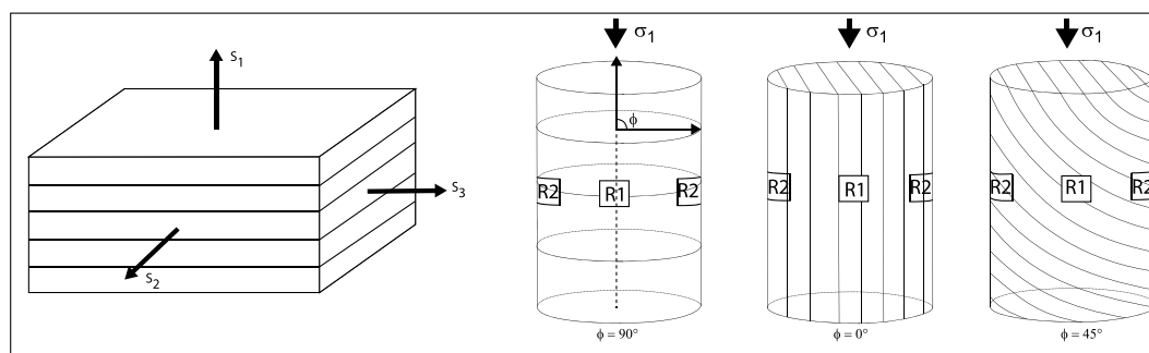
Figure 1. Coordinate system used to define the compliance matrix and tangent moduli. Sample configurations with angle \phi definition and strain gages location for each bedding orientation. Note that on each strain gage location, there is one axial and one radial strain gage.
