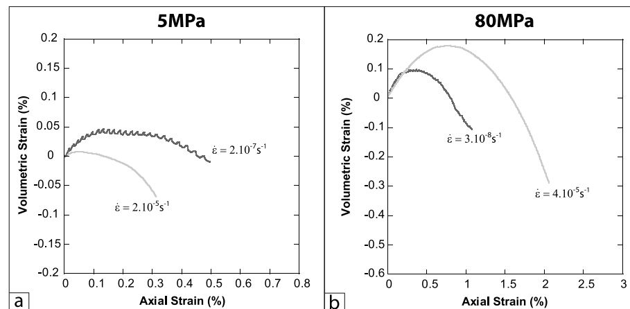
Figure 9. Volumetric strain (%) as a function of axial strain (%) for confining pressures of (a) 5 MPa and (b) 80 MPa and for bedding orientation \phi = 0^\circ , high strain rate (grey curve), and low strain rate (black curve).
