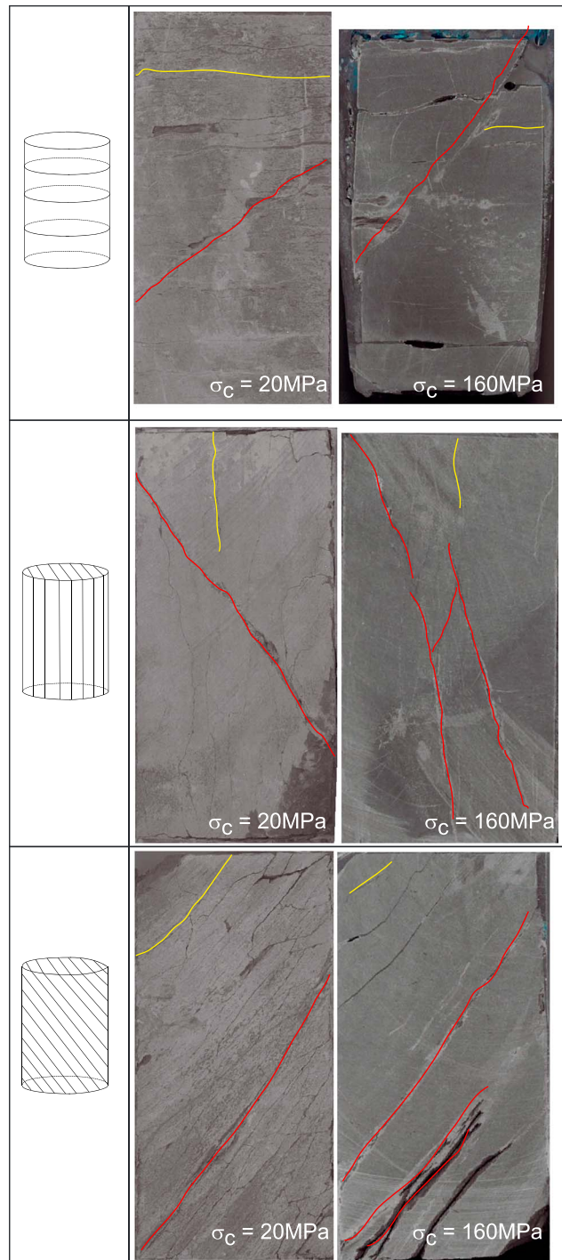
Figure 10. Postmortem images of fractured samples for confining pressures of (left column) 20 MPa and (right column) 160 MPa. Three bedding orientations are shown: (top row) \phi = 90^\circ , (middle row) \phi = 0^\circ , and (bottom row) \phi = 45^\circ , all deformed at low strain rate. The bedding orientation is highlighted in yellow, the fractures in red.
