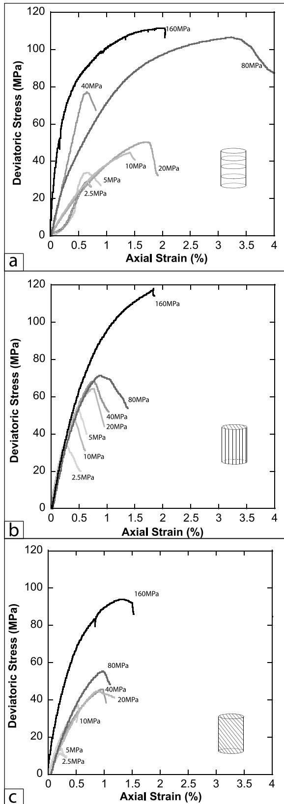
Figure 5. Deviatoric stress ( \sigma_1 - \sigma_3 , MPa) as a function of axial strain (%), for experiments performed along three bedding orientations: (a) \phi = 90^\circ , (b) \phi = 0^\circ , and (c) \phi = 45^\circ . Gray scale corresponds to the confining pressures investigated: 2.5, 5, 10, 20, 40, 80, and 160 MPa, from light grey for low confining pressures to black for high confining pressures.
