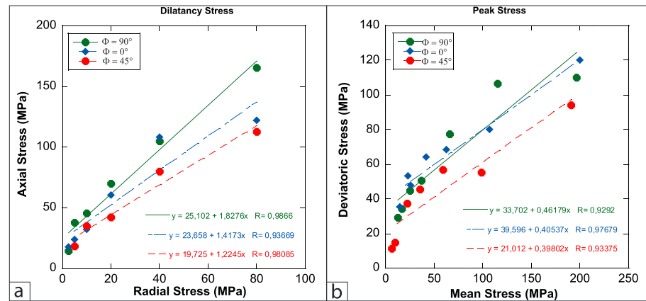
Figure 12. Fit of envelopes for (a) the transition to dilatancy in the radial stress-axial stress plane and (b) the peak stress in the mean stress-deviatoric stress plane.
