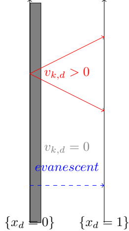
Figure 1: Apparence of the source term induced phases.
