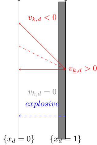
Figure 2: The first rebound.
