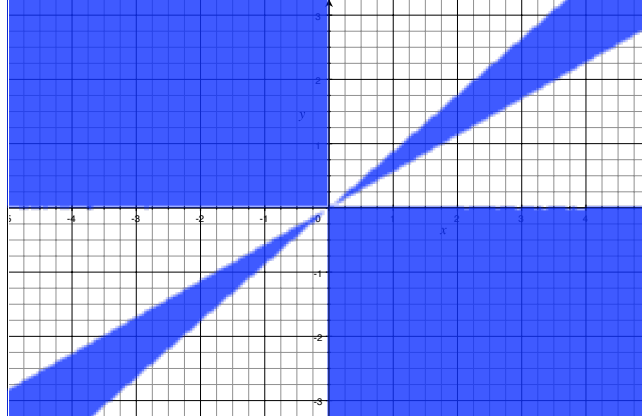
Figure 4: The set (in blue) of (x, y) \in \mathbb{R}^2 such that \left| \frac{y+x}{-y+x} \frac{-y+\alpha_0 x}{y+\alpha_0 x} + \frac{2xy}{\delta(-y+x)} \frac{\alpha_1}{y+\alpha_0 x} \right| < 1
