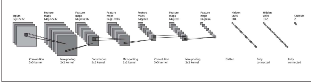
Figure 4. CNN used for classifying clouds. Structure is similar than the one used for the CIFAR-10 competition
