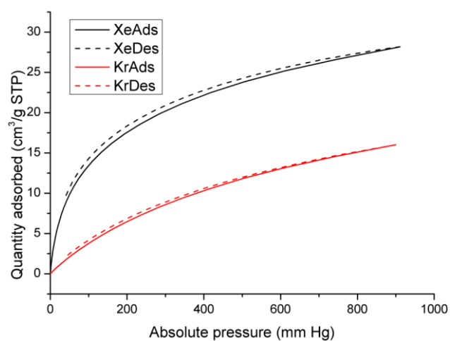
Figure 5: Isotherm curves (273.15 K) for the adsorption (solid) and the desorption (dash) of xenon (black) and krypton (red) in activated Product B .
