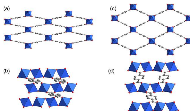
Figure 1: Structural views of the (a) and (b) closed (narrow pore) and (c) and (d) open (large pore) forms of the MIL-53 structure, with metal-centred octahedral shown in blue and the carbons of the 1,4-benzenedicarboxylate linker in grey. No guest molecules are shown.
