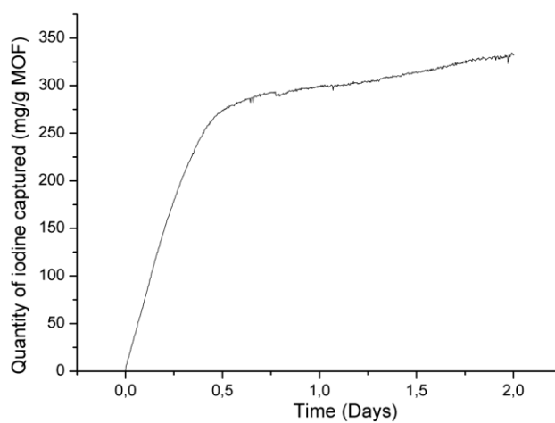
Figure 6: Iodine ( I_2 ) adsorption curve for activated Product B .
