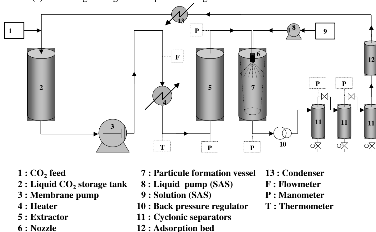
Figure 1 : Experimental set-up
