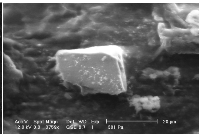
Figure 4: ESEM picture of a cocoa butter particle obtained with Exp # 5.
