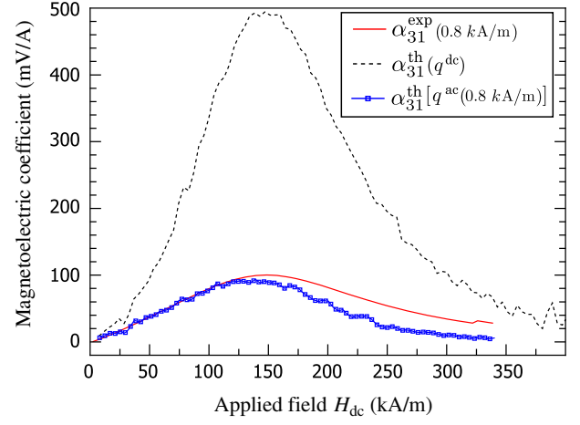
FIG. 6. Magnetoelectric coefficient measured for CFOA/PZT at H_{\text{ac}} \sim 0.8 kA/m and 80 Hz, compared to the calculated coefficient integrating either the measured strain derivative q^{\text{dc}} or the piezomagnetic coefficient q^{\text{ac}} at 0.8 kA/m.
