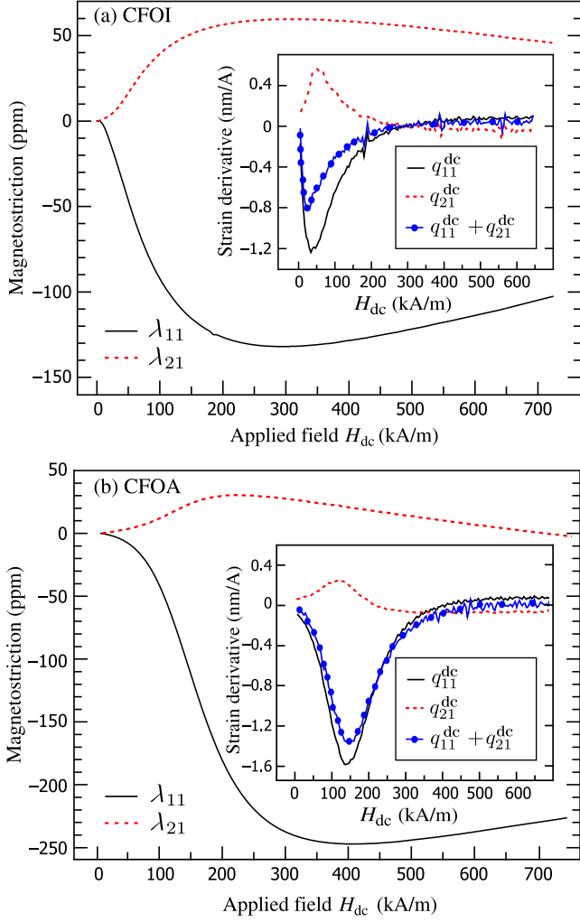
FIG. 3. Static longitudinal \lambda_{11} and transversal \lambda_{21} magnetostrictive curves for (a) CFOI and (b) CFOA. (Inset) The dc strain derivatives q^{\text{dc}} along the longitudinal and transversal directions, and the sum of the two.
