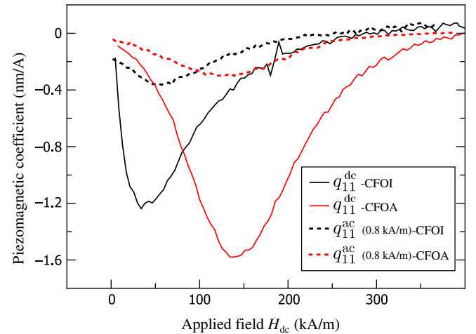
FIG. 4. Longitudinal strain derivative q_{11}^{\text{dc}} and piezomagnetic coefficient q_{11}^{\text{ac}} ( H_{\text{ac}} \sim 0.8 kA/m) for CFOI and CFOA.
