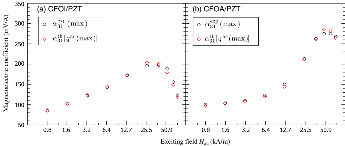
FIG. 7. The maximum magnetolectric coefficient measured \alpha_{31}^{\text{exp}} or calculated \alpha_{31}^{\text{th}} for ME bilayers (a) CFOI/PZT and (b) CFOA/PZT as a function of the excitation field H_{\text{ac}} at low frequency (80 Hz) (the semilog 2 plot). The calculated values integrate the measured piezomagnetic coefficients q^{\text{ac}} at each exciting field.
