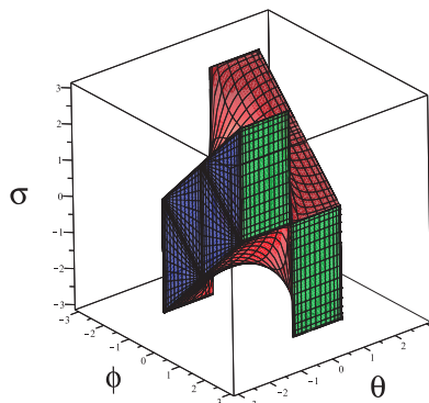
Fig. 3. The aspect of the 3-PPPS parallel robot around the “home” pose
