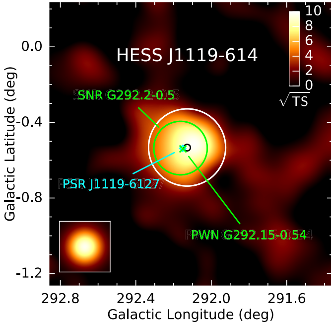
Fig. 18. Significance ( \approx \sqrt{TS} ) of the VHE \gamma -ray excess, centered on the new source HESS J1119–614, with the H.E.S.S. The PSF for this data set shown inset. The black circle at the center indicates the 68% uncertainty in the best-fit centroid of the VHE emission. The white circle represents the 70% containment region of the emission (R_SPEC, used also for spectral measurement). The approximate size of the radio shell of SNR G292.2–0.5 is shown as a green circle and the PWN G292.15–0.54 as a green marker. The position of the pulsar PSR J1119–6127 is denoted by a cyan diamond. The FoV is 1.5^\circ \times 1.5^\circ .
