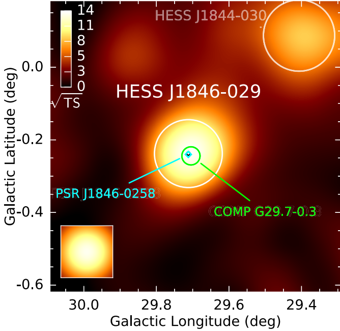
Fig. 30. VHE \gamma -ray image: HESS J1846–029. See Fig. 18 for a general description. Additionally, the composite SNR is shown by plotting a green circle approximating the radio shell. The position of the pulsar is indicated by a cyan diamond. The FoV is 0.8^\circ \times 0.8^\circ .
