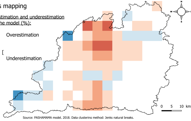
Fig. 2. Deforestation error by grid (in 1990)
