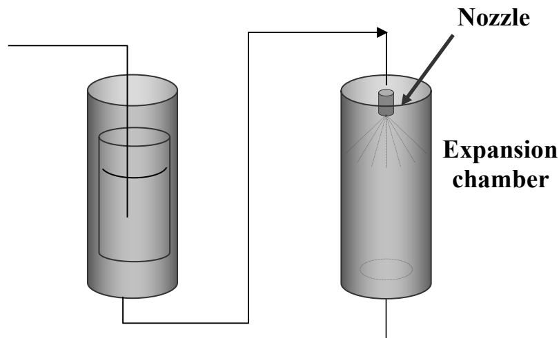
Figure 15. The PGSS process: schematic flow diagram
