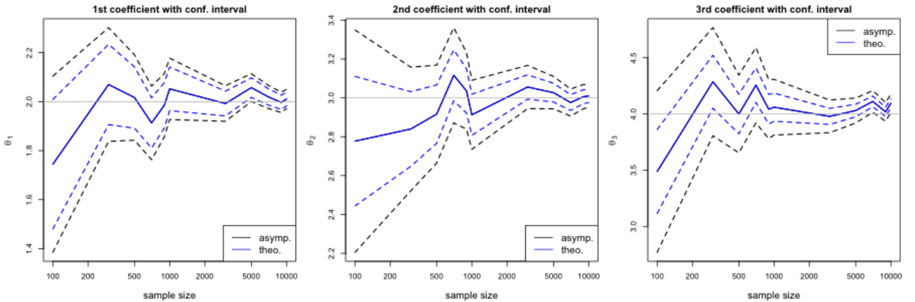
Figure 1: Estimated coefficient \hat{\vartheta}_{n,(2),i} in solid lines: blue for explicit formula and black for IWLS; dashed lines are corresponding confidence intervals
