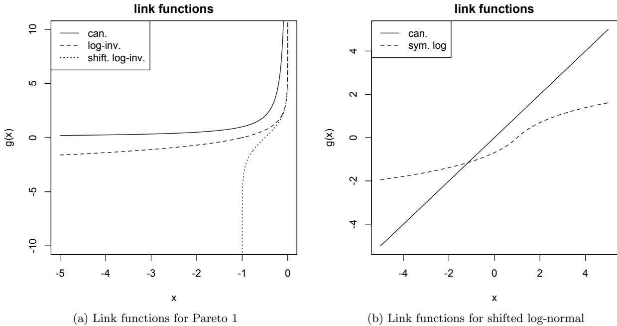
Figure 4: Graphs of link functions
