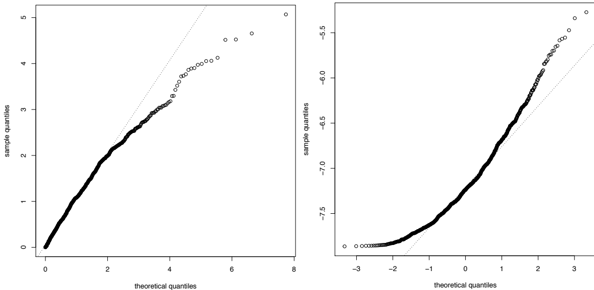
Figure 2: Quantile-quantile plots of the residuals defined in Section 4.3: (left) for pareto1, (right) for shifted log-normal
