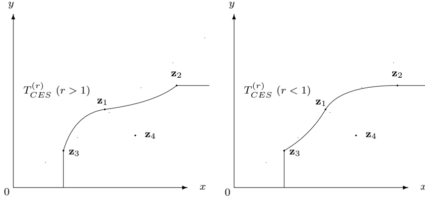
Figure 5.3 CES envelopment in the case r > 1 Figure 5.4 CES envelopment in the case r < 1
