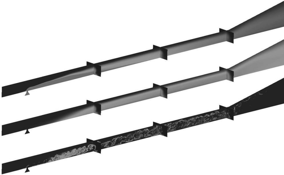
FIGURE 9. Combustion results from LES of the HyShot II combustor. Contours on a slice through the injector and three slices normal to the flow at x=80, 160 and 240 mm. Top: Mean mixture fraction from 0 to 0.1 (dark to light), where the stoichiometric mixture fraction is 0.028. Middle: Mean progress variable ( \text{H}_2\text{O} mass fraction) from 0 to 0.24 (dark to light). Bottom: Instantaneous source of progress variable on a logarithmic scale (dark to light).
