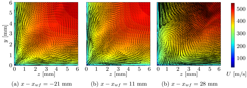
FIGURE 9. Downstream evolution (from LES) of corner flow in the vicinity of y = z = 0 , for stream-wise locations (relative to the wedge foot): x - x_{wf} = -21 , 11 and 28 mm (from left to right). Contours of mean stream-wise velocity, U , are superimposed with arrows representing the transverse velocity, V\mathbf{e}_y + W\mathbf{e}_z , where \mathbf{e}_\alpha is the versor in the \alpha -coordinate direction.
