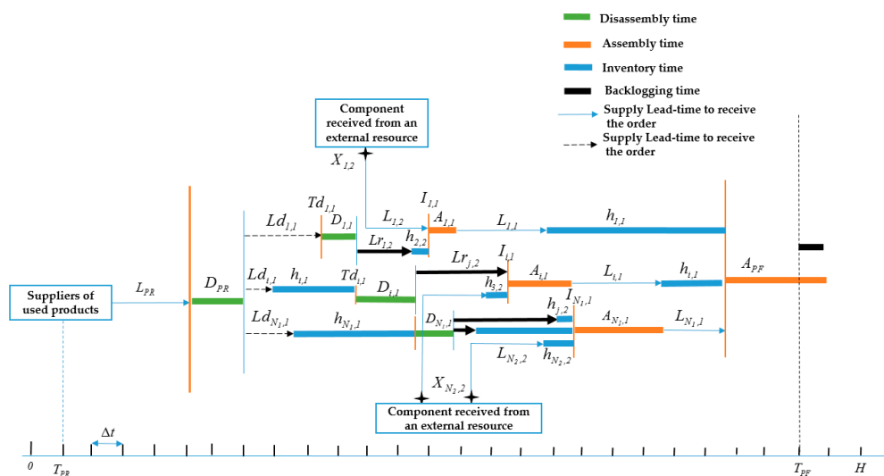
Figure 3. Description of one manufacturing finished product planning.
