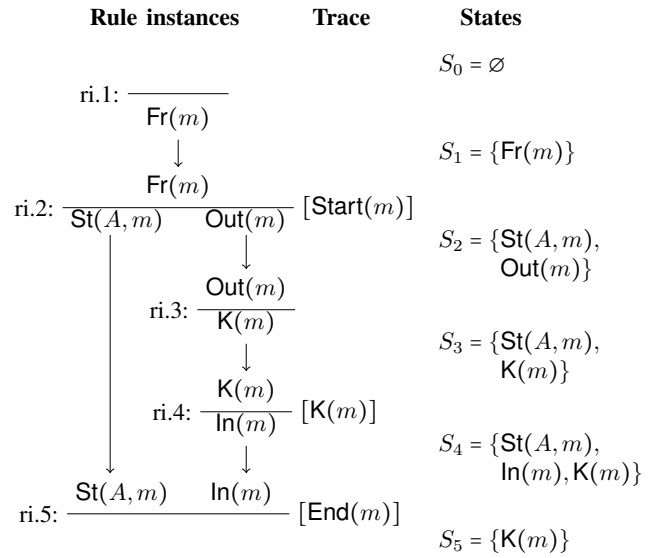
Fig. 2: Example execution of (P_{basic} \cup MD) .
