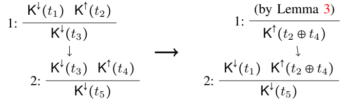
Fig. 13: Merging multiple deconstruction rule instances.
