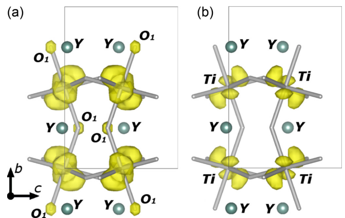
FIG. 1. Magnetization density reconstructed by maximum entropy method with (a) all measured reflections (the level of isodensity surface is 0.05 \mu_B / \text{\AA}^3 ) and (b) “special” reflections originating from the aspherical contribution of the Ti spin-density distribution (the level of isodensity surface is 0.10 \mu_B / \text{\AA}^3 ).
