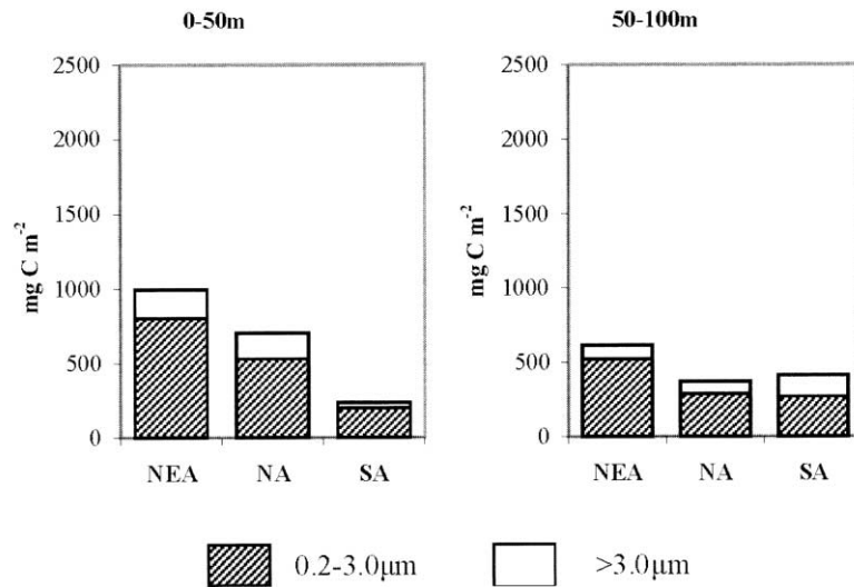
Fig. 4. Biomass distribution of autotrophs in the 0–50 and 50–100 m layers during March and September 1997.
