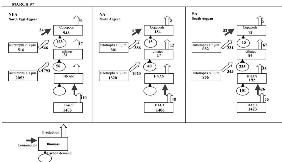
Fig. 7. Carbon budgets in March 1997. Numbers inside boxes show biomasses (mg C m -2 ); numbers inside ellipses show carbon demands (mg C m -2 day -1 ); numbers below the white arrows show productions (mg C m -2 day -1 ) and above black arrows show consumption (mg C m -2 day -1 ).
