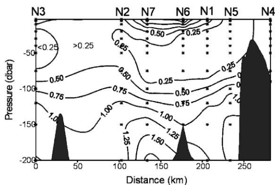
Fig. 3. Nitrate ( \mu\text{M} ) distribution in the sampling areas in March and September 1997.
