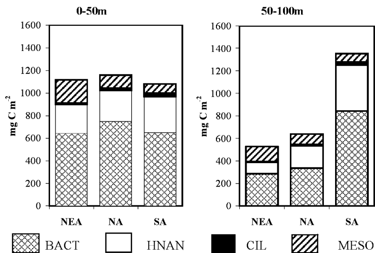
Fig. 5. Biomass distribution of heterotrophs in the 0–50 and 50–100 m layers during March and September 1997 (BACT=bacteria, HNAN=heterotrophic nanoflagellates, CIL=ciliates, MESO=mesozooplankton).
