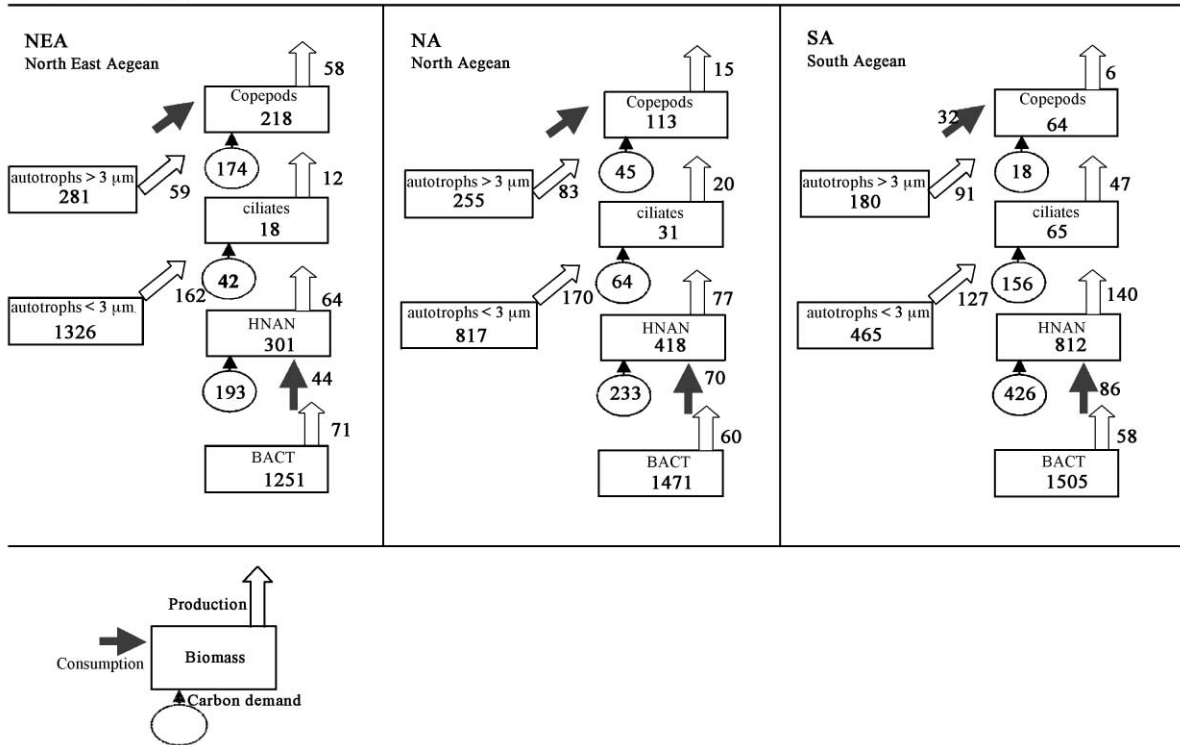
Fig. 8. Carbon budgets in September 1997.
