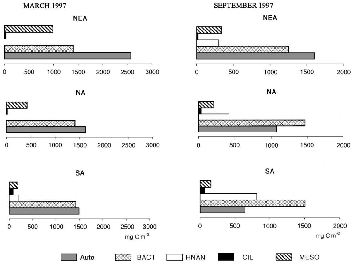
Fig. 6. Carbon partitioning among auto- and heterotrophs in March and September 1997. Auto: autotrophic biomass; BACT: heterotrophic bacteria; HNAN: heterotrophic nanoflagellates; CIL: ciliates; MESO: mesozooplankton.
