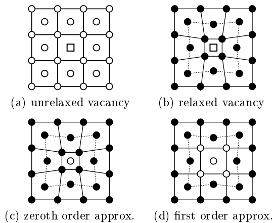
FIG. 4. Schematic illustration of the procedure used for the computation of the Kanzaki forces in the case of a vacancy defect. The white spheres correspond to atoms at their perfect bulk positions, i.e. before relaxation, the white square to the vacancy defect, and the black spheres to the atoms at their relaxed position around the defect.
