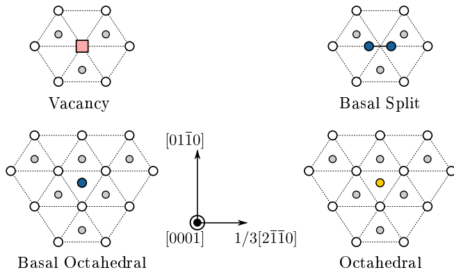
FIG. 1. Projection in the basal plane of the different point-defects investigated in hcp Zr: the vacancy and three SIA configurations. The white spheres represent the bulk Zr atoms at z = 0 , the grey spheres the bulk Zr atoms at z = c/2 . The square represents the vacancy (V), the blue spheres are SIAs at z = 0 (BO and BS configurations), and the yellow sphere the SIA at z = c/4 (O configuration).
