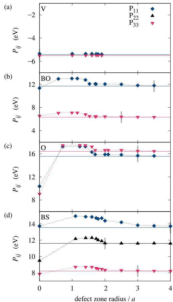
FIG. 6. Convergence of the elastic dipole components with the radius of the defect restoration zone for the Kanzaki method. The elastic dipoles are calculated for the vacancy and the BO, O and BS configurations of the SIA, using EAM #3 potential. The horizontal lines indicate the values deduced from the residual stress method. The vertical gray ticks indicate the converged values of the defect restoration radii, corresponding to the point-defect core zone dimensions.
