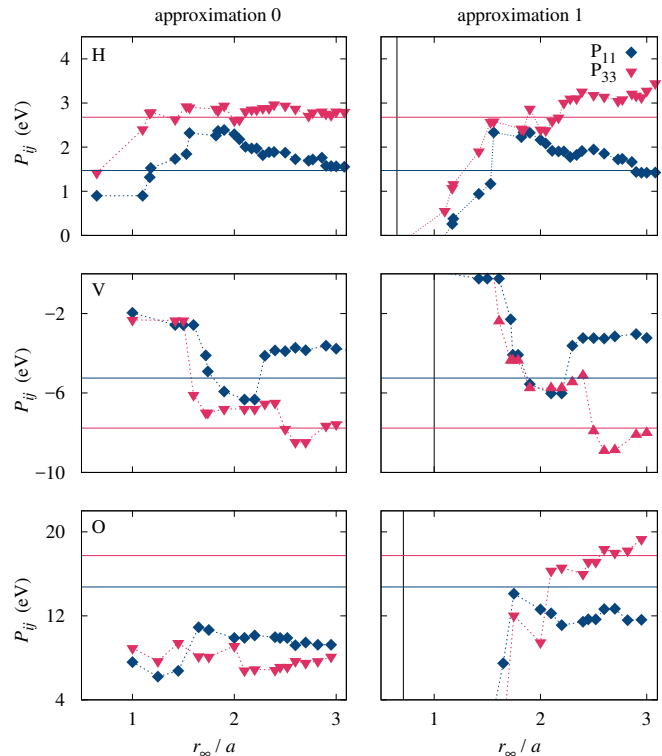
FIG. 7. Convergence of the elastic dipole components obtained from the Kanzaki forces with the cutting radius r_\infty of the force summation (Eq. 4), for the H solute atom, the vacancy, and the O configuration of the SIA, computed using ab initio calculations. When computing the Kanzaki forces, only the point-defect is restored in the left figures (approximation 0), whereas the first neighbor shell is also restored in the right figures (approximation 1). The horizontal lines indicate the values deduced from the residual stress and the vertical lines the radius of the restoration zone.
