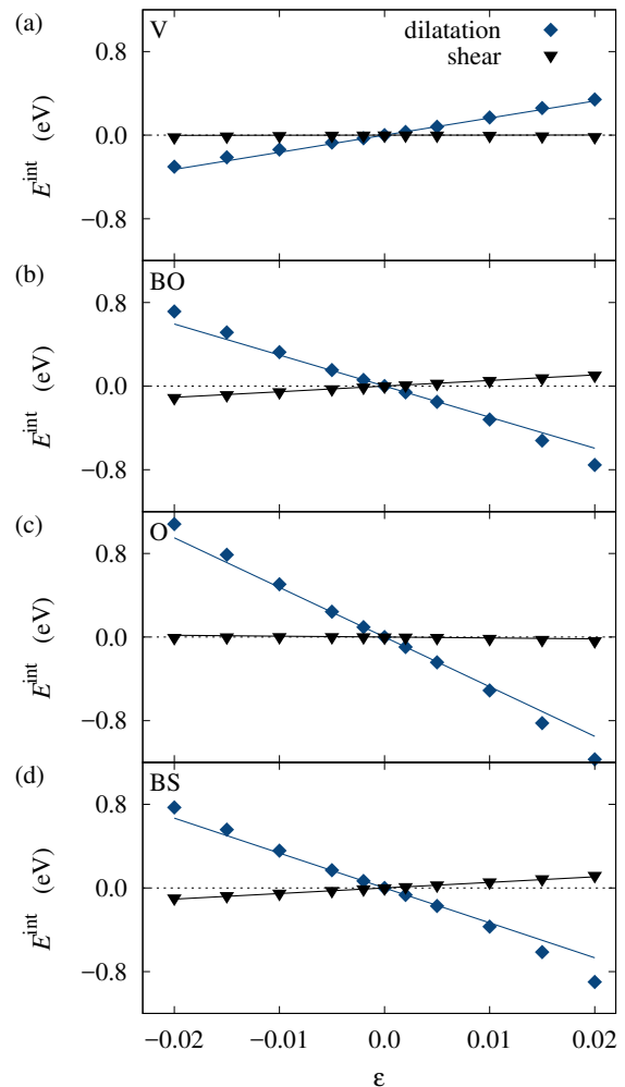
FIG. 2. Interaction energy between (a) V, (b) BO, (c) O and (d) BS point-defects and homogeneous applied strains corresponding either to dilatation or pure shear. Filled symbols are the results of atomistic simulations and straight lines the predictions of elasticity theory (Eq. 5) using the elastic dipole deduced from the residual stress (Eq. 8). Data have been obtained with the EAM #3 potential.
