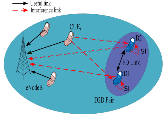
Fig. 1. A FD-D2D pair shares the resources of one cellular user, which creates interference between the two types of links.
