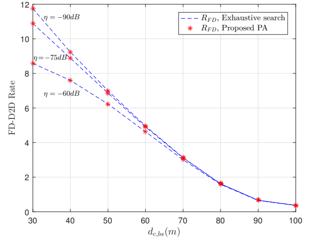
Fig. 4. Comparison of FD-D2D rate obtained from the exhaustive search and from the proposed power allocation scheme in the symmetric case
