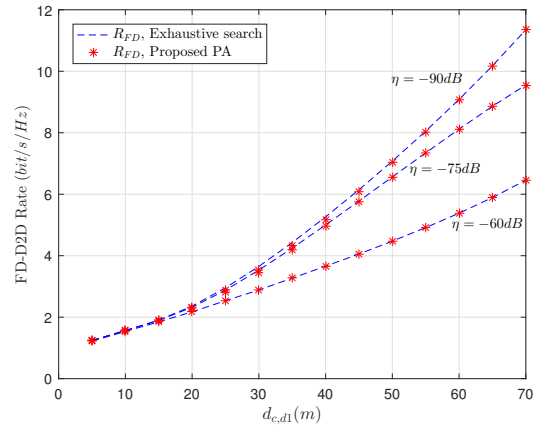
Fig. 5. Comparison of FD-D2D rate obtained from the exhaustive search and from our proposed power allocation scheme in the asymmetric case
