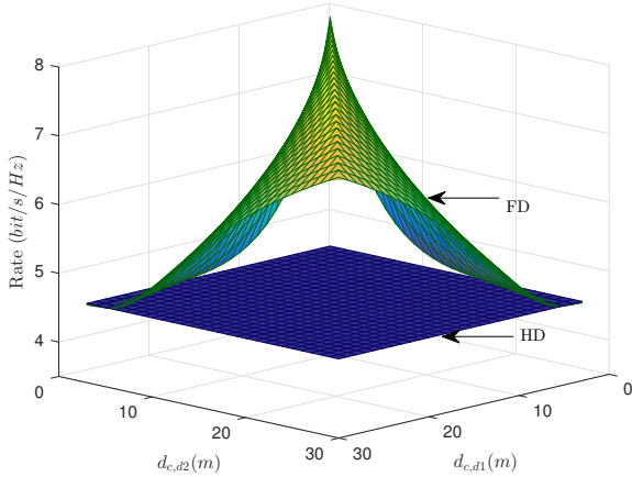
Fig. 7. The effect of the CUE location on the FD rate. ( \eta = -70\text{dB} )
