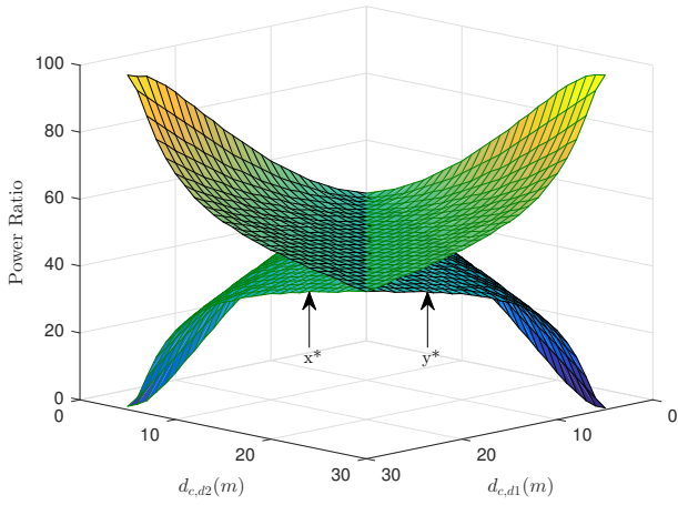
Fig. 6. The optimal power ratios variation w.r.t to CUE location. ( \eta = -70\text{dB} )
