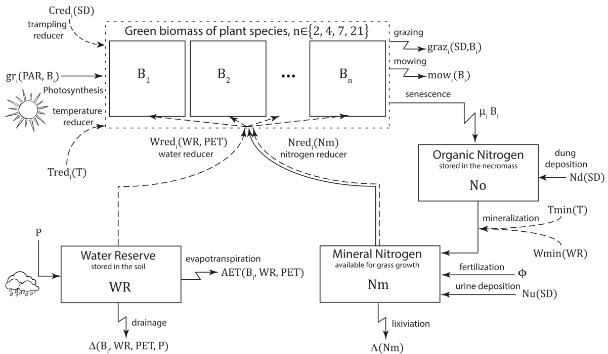
169 170 Fig. 1 Structure of the DYNAGRAM model. Solid lines denote flows of matter or energy and 171 dashed lines denote reducers (mineral nitrogen acts both as a flow and as a reducer). State 172 variables and forcing climatic variables are listed in Table 1 and a description of all 173 parameters can be found in Tables A.1 and A.2 (Appendix A).
