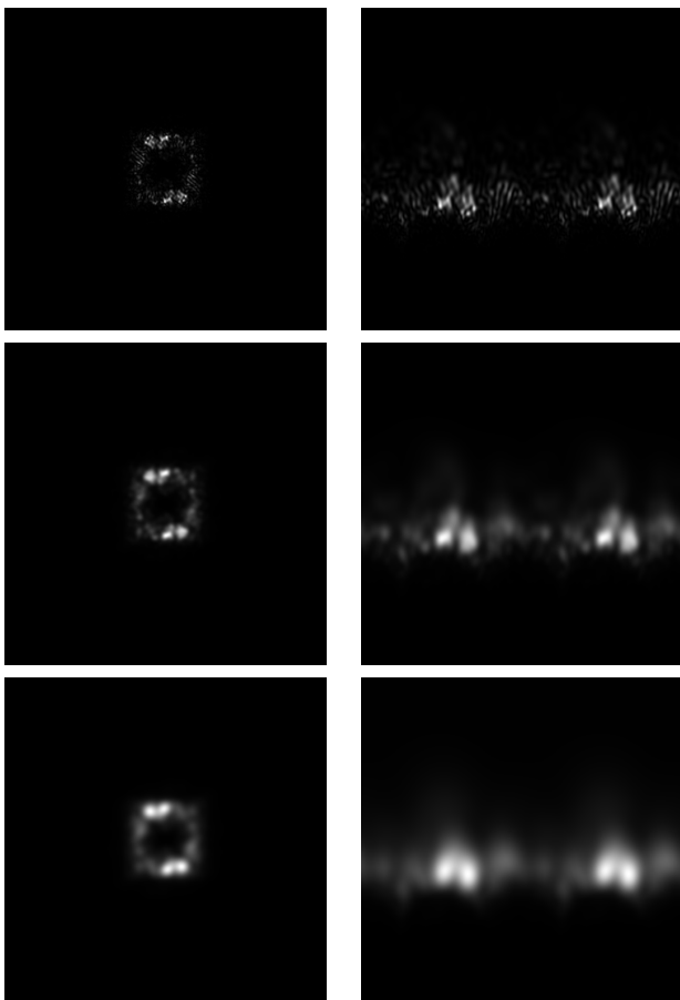
Fig. 7. PSD estimated using the square of the modulus of the Discrete Fourier Transform. 1st row: left, periodogram with size 512 \times 512 obtained using zero-padding method (PSD1); right, interpolated PSD1 in polar coordinates. 2nd row: left, PSD1 smoothed by a Gaussian filter with \sigma = 3 (PSD2); right, interpolated PSD2 in polar coordinates. 3rd row: left, PSD1 smoothed by a Gaussian filter with \sigma = 6 (PSD3); right, interpolated PSD3 in polar coordinates.
