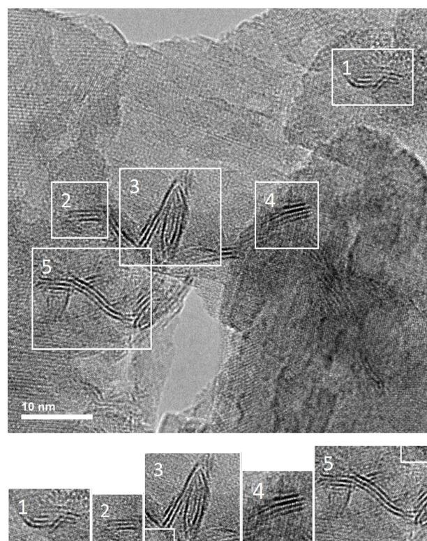
Fig. 1. Molybdenum sulfide sheets (black fringes) deposited on an alumina support (top image) and its sub-images (significant fringes selected, in the second row). The initial image consists of 1024 \times 1024 pixels. The numerical resolution is 0.057 nm by pixel.
