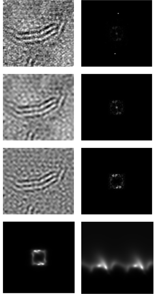
Fig. 4. ARFBF modeling of HRTEM image. In the first row, the original image I_1 and its PSD S_1 ; in the second row, the image I_2 (after WHFR pre-processing) and its PSD S_2 ; in the third row, the image I_3 (after removing the FBF contribution from the image I_2 ) and its PSD S_3 . Finally, the last row presents the PSD calculated with the parameters estimated by AR modeling in Cartesian coordinate (left) and in polar coordinate (right - lines are associated with radii and columns to angles).
