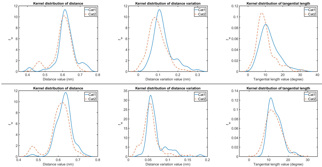
Fig. 6. Kernel distributions of distance (left), distance variation (center) and tangential length (right) of the detected lobe S_{LobeD}^* of Cat 1 (— in blue) and Cat 2 (--- in red). First row: using PSD estimated in polar coordinates with HM method based on the AR model. Second row: Using interpolated periodogram in polar coordinates.
