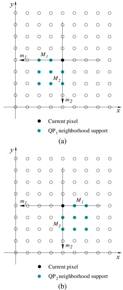
Fig. 2. Quarter plan prediction supports denoted (a) D_{QP_1} (Eq. 3) and (b) D_{QP_2} (Eq. 4) with finite order (M_1, M_2) = (2, 2) and (x, y) \in \mathbb{Z}^2 .
