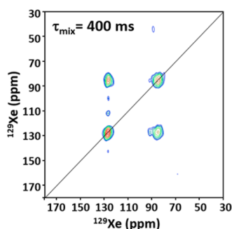
Figure 7. 2D ^{129}\text{Xe} MAS EXSY spectrum of MIL-53(Al) loaded with xenon and recorded at \nu_{\text{R}} = 10 kHz and room temperature with \tau_{\text{mix}} = 400 ms.
