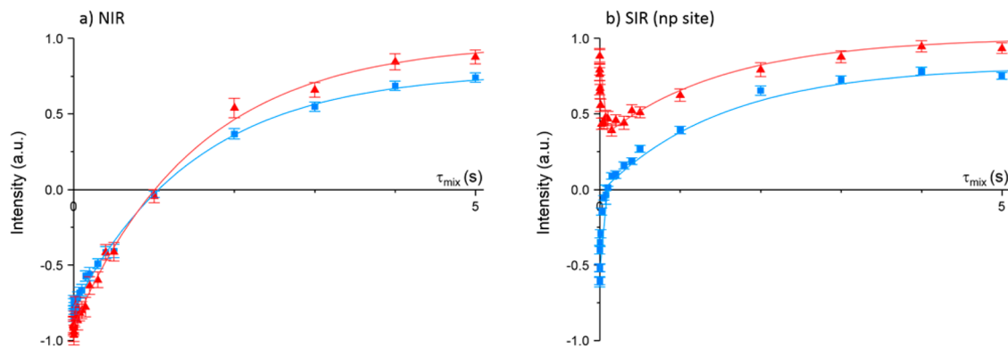
Figure 8. (a) NIR and (b) SIR experiments on MIL-53(Al) loaded with xenon at \nu_{\text{R}} = 10 kHz and room temperature. For SIR experiment, the np signal was selectively inverted. The experimental signal intensities are displayed as symbol (blue squares for np form and red triangles for lp one). The best fit curves are displayed as continuous lines (blue for np form and red for lp one). The error bars were taken as the noise standard deviation of the signals.
