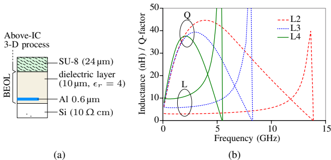
Fig. 4. (a) layers added under above-IC solenoids, (b) simulated data of above-IC solenoids L_2 (---), L_3 (····) and L_4 (—) versus frequency.
