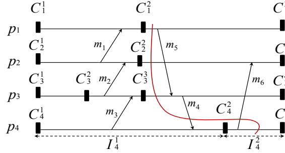
Figure 2: A communication and checkpoint pattern with a possible crash scenario
