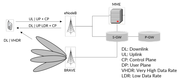
Fig. 1. Example of Kiosk application with offloading. The very-high data rate services are transmitted using the mmW downlink, while the others services (including control plane) are allocated to 4G/5G cellular network.
