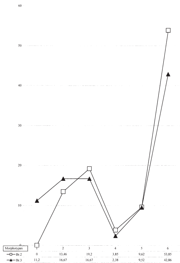
Fig. 13: Château Breccia, Arvicola cantianus : Distribution of the morphotypes (position of the Mimomys -fold) within group A (Breccia 2) and group B (Breccia 3).
