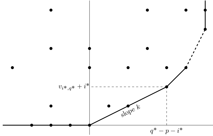
FIGURE 1. Definition of the pair (i^*, q^*) .
