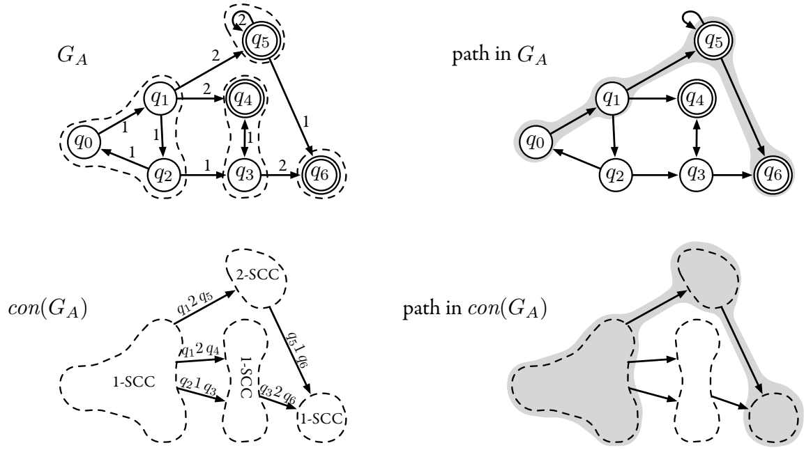
Figure 2: Example of path in G_A and corresponding path in con(G_A) . For simplicity, we assume that the alphabet is singleton \mathbb{A} = \{a\} , and we therefore omit ‘ a ’ in the transitions.
