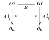
Figure 2: Simplification step
