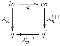
Figure 1: Completion step
