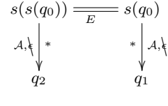
Figure 3: Implication example
