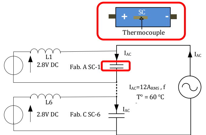
Fig. 4 Scheme of the experimental test bench
