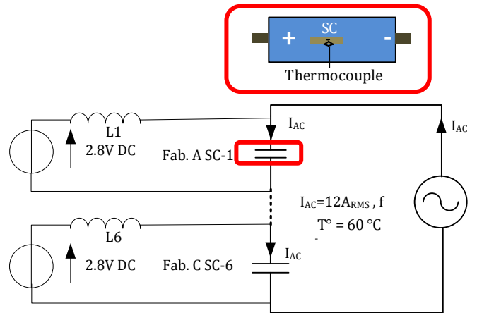
Fig. 4 Scheme of the experimental test bench
