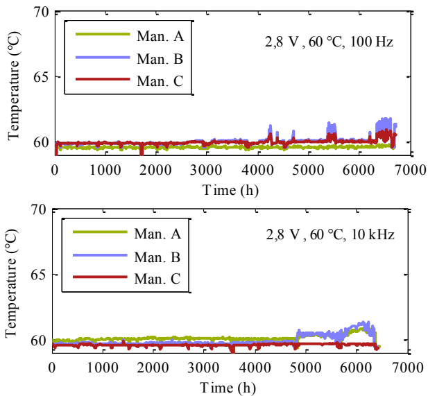
Fig. 6 Evolution of temperature for 100 Hz and 10 kHz ripple current
