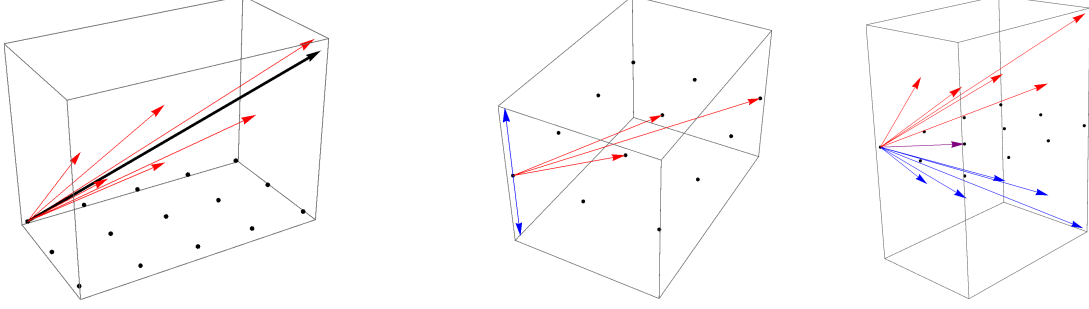
Figure 5: Left: Applying Proposition 2.3 to a vector (black) with \varepsilon = 0.1 , in dimension 3, yields the red offsets. Center: Discretization stencil for the Reeds-Shepp model, red offsets obtained by applying Proposition 2.3 in dimension d = 2 , blue offsets related to the angular dimension. Right: Stencil for Dubins model, red and blue offsets obtained by applying Proposition 2.3 in dimension d = 3 to two distinct vectors.
