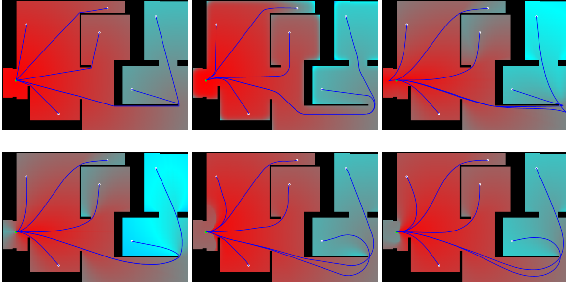
Figure 24: Optimal paths coming from various models. The green point is the source, the white points are endpoints, black parts indicate the walls and the color indicates the distance (if necessary minimized over orientation). Top row, left to right: isotropic, isotropic with cost based on Gaussian blurred image, Reeds-Shepp model. Bottom row, left to right: Forward-only Reeds-Shepp model, Dubins's model, Euler-Mumford elastica model.
