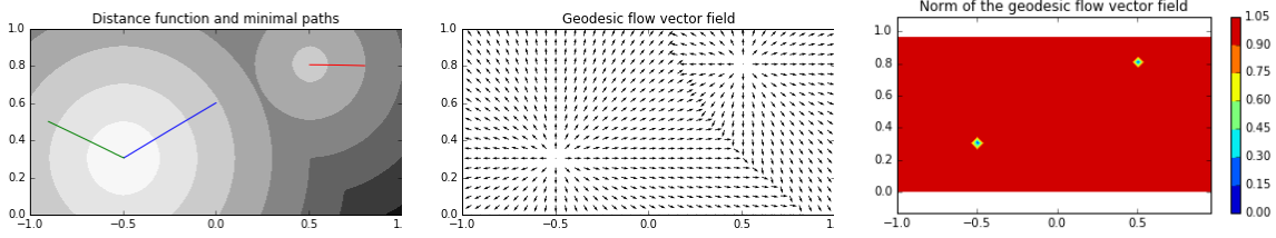
Figure 10: Left: distance map u(\mathbf{p}) := \min\{|\mathbf{p} - \mathbf{p}_1|, \sigma_2 + |\mathbf{p} - \mathbf{p}_2|\} , where \mathbf{p}_1 = (-0.5, 0.3) , \mathbf{p}_2 = (0.5, 0.8) and \sigma_2 = 0.5 , numerically computed using isotropic fast marching with second order enhancement. Center: geodesic flow V(x) := \nabla u(x) obtained numerically using (39). Right: verification that |\nabla V(x)| = 1 , at all points of differentiability.
