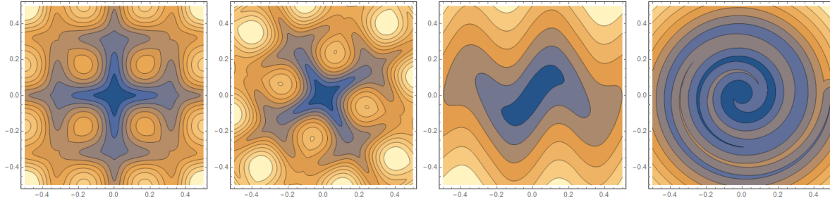
Figure 17: Level sets of the four 2D anisotropic Riemannian examples described in §4.3.
