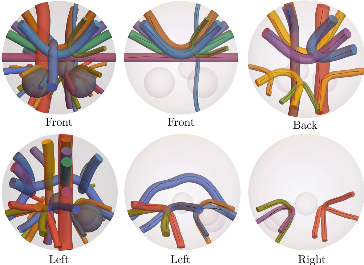
Figure 9: Visualization of the ISBI dataset from different viewpoints. The two left-most images show the full dataset, the other four images show a selection of the bundles. The black lines inside these bundles indicate the geodesics obtained with fast marching.
