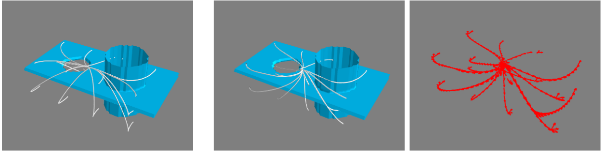
Figure 22: Left: Motion planning with the three-dimensional Reeds-Shepp model, with configuration space \mathbb{R}^3 \times \mathbb{S}^2 . Note the cusps , where the vehicle orientation is reversed. Center: Likewise, but with the Reeds-Shepp forward variant. Right: orientations for the forward model, note the in place rotations at some of the path endpoints.
