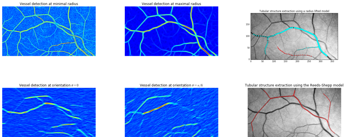
Figure 25: Vessel segmentation in an image of the retina, using two dimension lifting techniques. Top: In a radius-lifted model, a preliminary image filtering is used to detect vessels of small (left) and large (center) scale. The backtracked path contains information about the vessel radii (right). Bottom: In an orientation lifted model, a preliminary image filtering detects vessel bits of different orientations (left and center). Vessel extraction using the Reeds-Shepp model (right).
