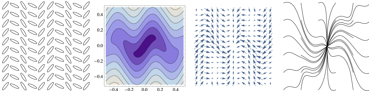
Figure 1: The four steps of minimal path computation. (I) Define a metric, here of Riemannian type and visualized as a family of ellipsoids. (II) Compute of a distance map, here from the center point, by solving the eikonal PDE (3). (III) Compute the geodesic flow direction \mathbf{p} \in \Omega \mapsto d\mathcal{F}_{\mathbf{p}}^*(du(\mathbf{p})) . (IV) Backtrack the minimal geodesics, by solving the ODE (5).
