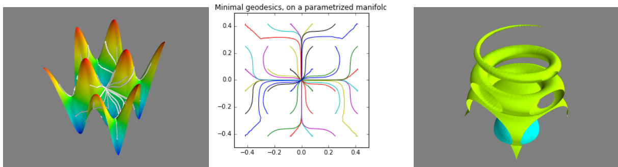
Figure 16: Left: Minimal geodesics on a parametrized surface in \mathbb{R}^3 . Center: Top view of the same geodesics. Right: Level sets of the front, for a test case inspired by three dimensional tubular structure segmentation.
