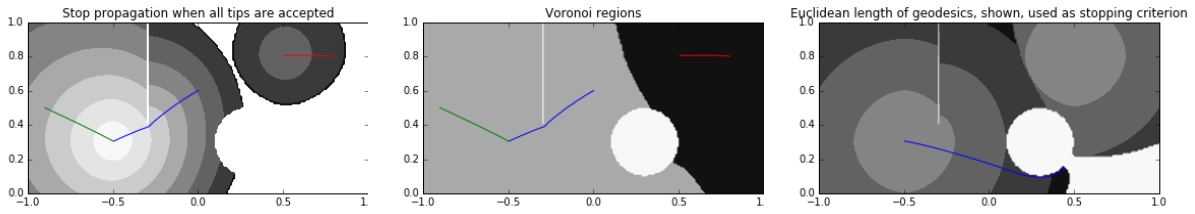
Figure 12: Left: Front propagation stopped when all geodesics tips are accepted, which is enough for backtracking. Center: Voronoi regions associated with the two seeds. Right: The Euclidean length l(\mathbf{p}) of the minimal path from each point \mathbf{p} \in \Omega , shown here, can be computed simultaneously with the distance map u(\mathbf{p}) . It is used as a stopping criterion in this experiment.
