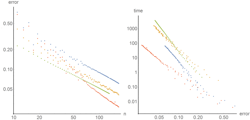
Figure 7: Comparison of the resolution/accuracy (left) and accuracy/computation time (right) compromise of several numerical methods for the eikonal equation of the Reeds-Shepp model. Log-log scale. In both figures we compare an iterative approach (green), the FM-LBR (yellow), the FM-VR1 implemented in the HFM-library (blue), and the same with second order enhancement (red). The latter turns out to be the most efficient, see §4.4 for a discussion.
