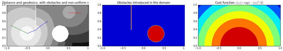
Figure 11: Distance map obtained using isotropic fast marching (left), in the presence of obstacles (center), and of a non-constant cost function (right, level sets shown).
