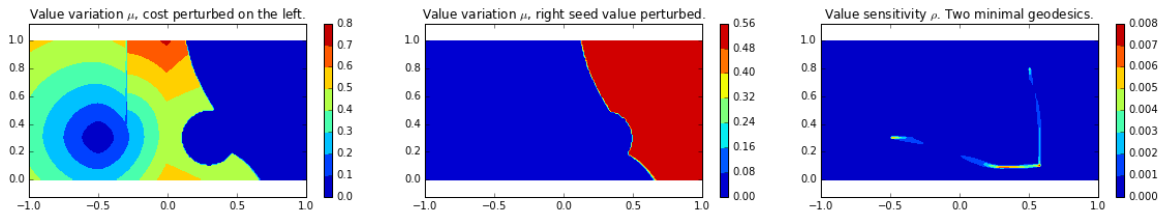
Figure 14: Left: First order term \mu in the Taylor expansion u_\varepsilon = u_0 + \varepsilon\mu + o(\varepsilon) of the distance map associated with the perturbed cost c_\varepsilon = c_0 + \varepsilon\chi_{x<0} . Center: Likewise, for a perturbation of the boundary condition \sigma_{2,\varepsilon} = \sigma_2 + \varepsilon at the seed \mathbf{p}_2 = (0.5, 0.8) . Right: Sensitivity \phi , with respect to the cost function, of the distance map u(\mathbf{p}_*) at a point \mathbf{p}_* . The support of \phi approximates the minimal geodesic(s) from \mathbf{p}_* to the seed points. Two geodesics are visible here since \mathbf{p}_* was chosen in the cut locus.
