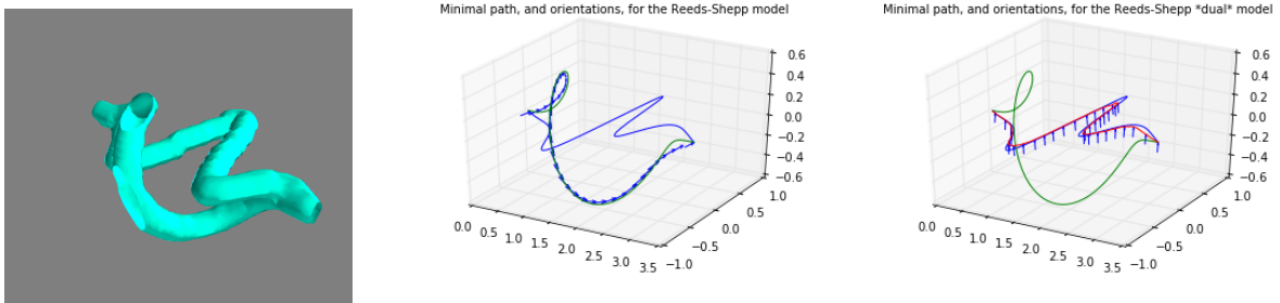
Figure 21: Left: Level set of the cost function, depending on the physical position only c = c(\mathbf{x}) , and which is small in the neighborhood of two curves, with respectively low torsion and low curvature. Center: The minimal path backtracked with the Reeds-Shepp model on \mathbb{R}^3 \times \mathbb{S}^2 follows the low curvature curve. Right: The minimal path backtracked with the Reeds-Shepp dual model follows the low torsion curve. A point \gamma(t) = (\mathbf{x}(t), \mathbf{n}(t)) of the backtracked path is represented by an arrow with origin \mathbf{x}(t) and direction \mathbf{n}(t) .
