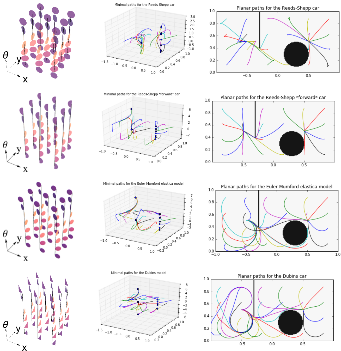
Figure 18: From top to bottom: Reeds-Shepp, Reeds-Shepp forward , Euler-Mumford elastica, and Dubins car models. Left: Control sets, i.e. unit balls of the local metric. Center: Minimal paths in \mathbb{R}^2 \times \mathbb{S}^1 . Right: Planar projection of the minimal paths.
