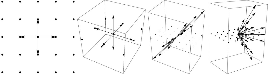
Figure 3: The stencil of a PDE numerical scheme is the collection of offsets, towards close neighbors usually, involved in its definition. We display the stencils used for the discretization of eikonal equations, associated with (left, center left) an isotropic metrics in dimension 2 and 3, (center right) an anisotropic Riemannian metric, (right) the Euler-Mumford elastica model.
