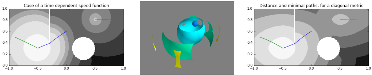
Figure 13: Distance map associated with, respectively: a time dependent cost function (left), a three dimensional isotropic metric (center), or a diagonal metric (right).
