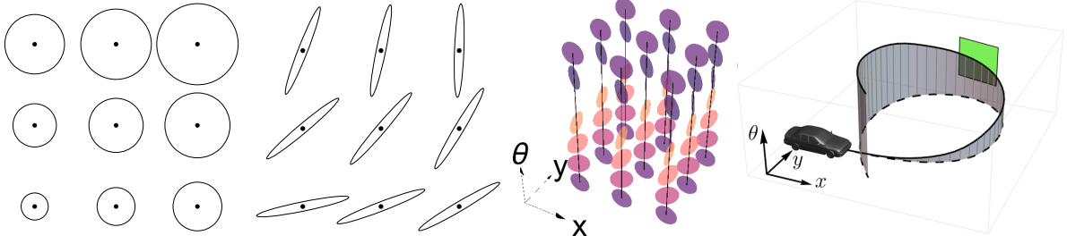
Figure 2: A metric associates to each point a gauge, i.e. a generalized norm which may be non-symmetrical and may take infinite values. The three first figures display unit balls (also referred to as Tissot's indicatrix) of the gauges of successively: an Isotropic metric, an Anisotropic Riemannian metric, and the non-holonomic sub-Riemannian metric associated with the Reeds-Shepp model on \mathbb{R}^2 \times \mathbb{S}^1 . In the later case, the admissible directions of motion depend on the present angular coordinate \theta , associated with the vertical axis, reflecting the fact that a car cannot move sideways.
