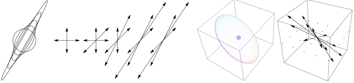
Figure 4: Dual unit ball \{\hat{\mathbf{p}}; \|\hat{\mathbf{p}}\|_{D^{-1}} \leq 1\} , and offsets associated by Voronoi’s first reduction to a tensor D , involved in the decomposition (23). Left: several examples in dimension two. Right: a three dimensional case.
