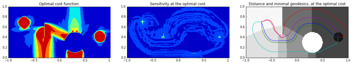
Figure 15: Left: Cost function maximizing the distance between the seed (-0.7, 0.7) and tip \mathbf{p}_* = (0.8, 0.4) , subject to bound constraints and a mean penalty, see (45). Center: Sensitivity of u(\mathbf{p}_*) w.r.t. the cost function, at the optimum. Right: Distance map u from the seed, backtracked geodesics from the tip \mathbf{p}_* and nearby pixels, at the optimum.
