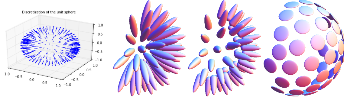
Figure 8: Left: Discretization of the unit sphere \mathbb{S}^2 , using 24 \times 12 points, used for the presented numerical experiments in \mathbb{R}^3 \times \mathbb{S}^2 . The next three pictures show the sets \{\dot{\mathbf{x}} \in \mathbb{R}^3; \mathcal{F}_{(0,\mathbf{n})}^\varepsilon(\dot{\mathbf{x}}, 0) \leq 1\} , with the relaxation parameter \varepsilon = 0.2 and for several orientations \mathbf{n} \in \mathbb{S}^2 , where \mathcal{F} is successively the metric of the Reeds-Shepp model (needles), of the forward variant (half needles), and of the dual variant (plates).
