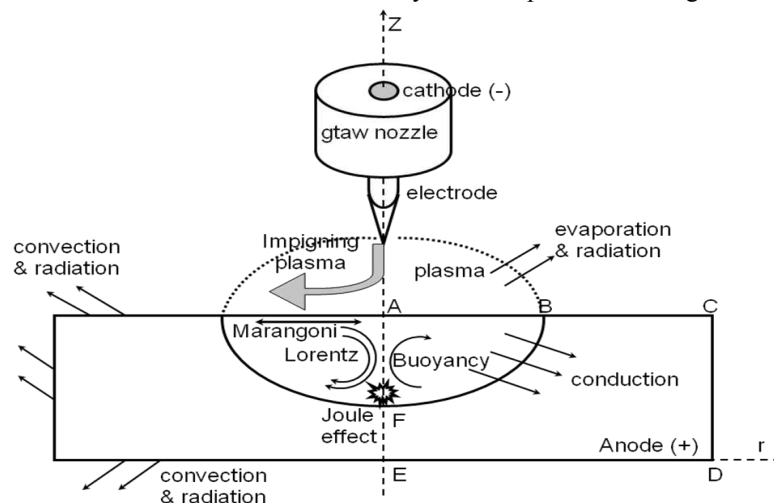
Figure 1: Schematic of transport phenomena occurring in the GTA Welding process
