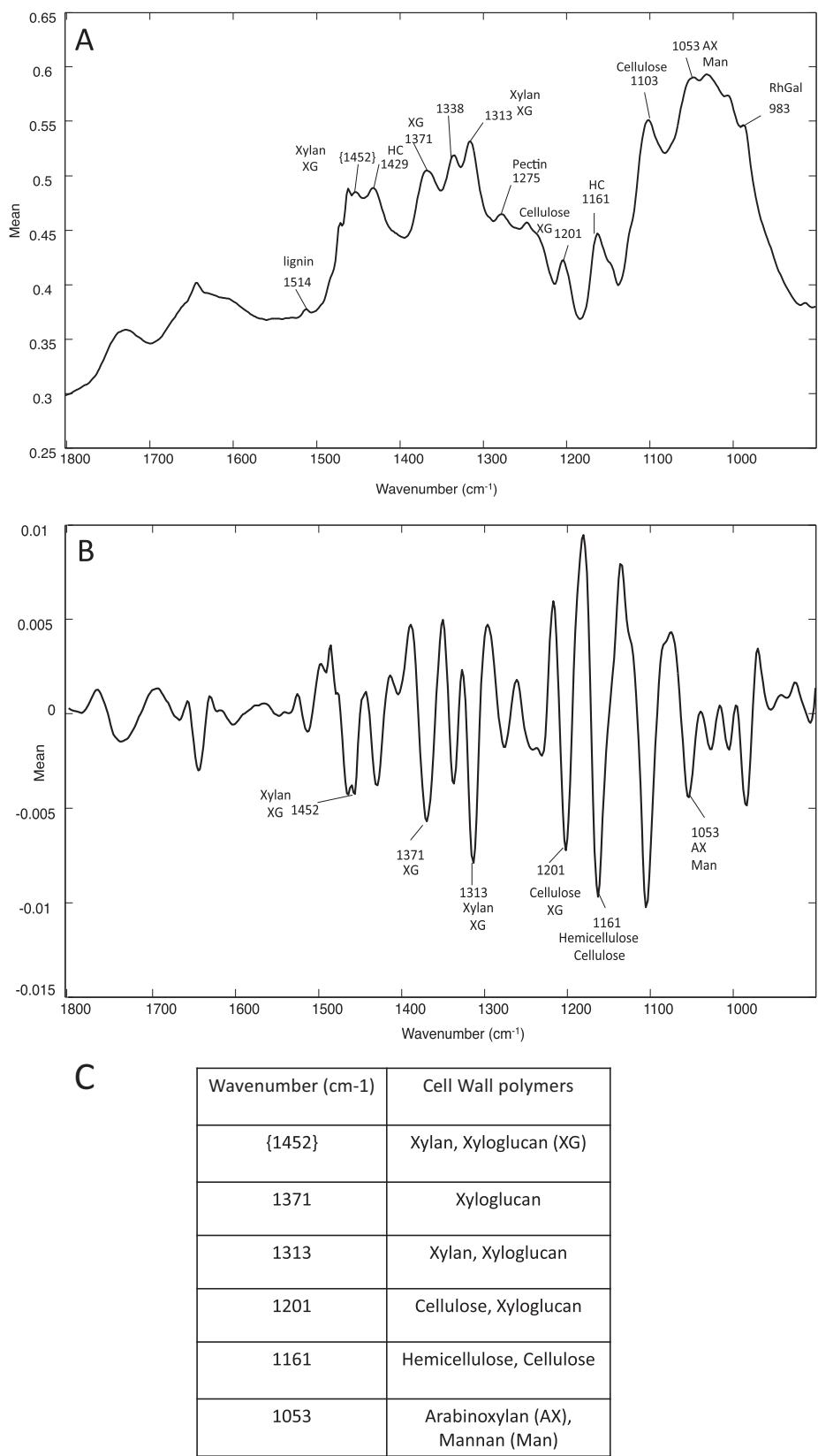
FIG. 8. Middle infra-red spectra at 1800–900 \text{cm}^{-1} of bast fiber cell walls (A) and secondary derivative (B) showing significant peaks characteristic of hemicelluloses (C).
