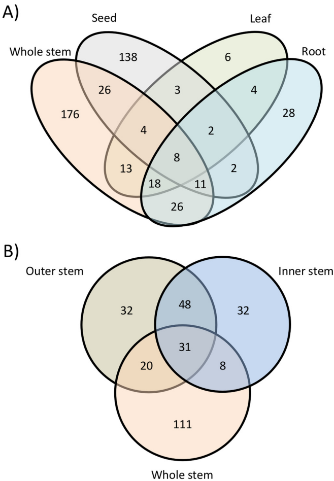
FIG. 3. Repartition of the 465 flax Total CWP identified in 4 different organs (A) and stem tissues (B). Whole stem (WS), Seeds (S), leaves (L), roots (R), Inner stem (IS), Outer stem (OS).
