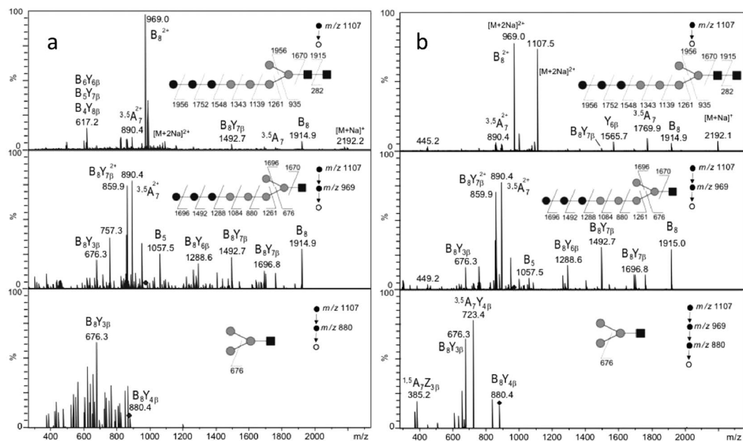
Figure 6. ESI-MS n spectra with n = 2 (upper panel), n = 3 (middle panel + lower panel (a)) and n = 4 (lower panel (b)) of permethylated LLO derivative ( m/z 1107 corresponding to [M + 2Na]^{2+} precursor ion) from lipid-linked oligosaccharides of cw92 C. reinhardtii cells (a) and the YG170 yeast mutant cells (b). On each panel, the precursor ion selected for the fragmentation analysis is shown with a diamond and its fragmentation pattern is proposed. Black square: GlcNAc; grey circle: Man; black circle: Glc.
