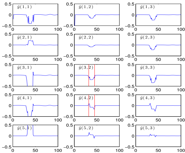
Fig. 10. Residual signal based on \{y_2, y_3\}
