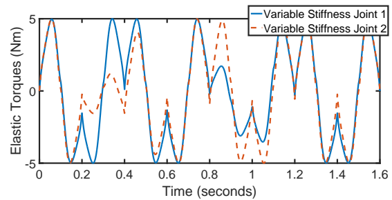
Figure 9: INPUT TORQUES FOR THE JOINTS OF VARIABLE STIFFNESS, 0.2 s AS PICK-AND-PLACE TRAVEL TIME BETWEEN DESIRED POINTS.
