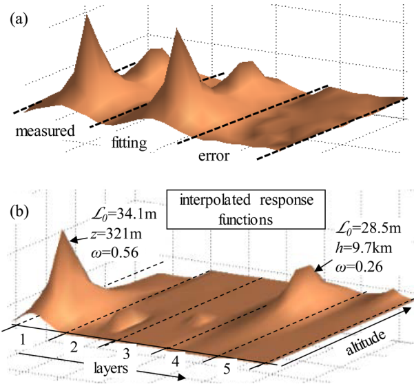
Figure 7. Fitting C_{\text{rsp}}(\mathcal{L}_0, h) functions to C_{\text{meas}} (from on-sky data, 2013 May 22 02:41:12): (a) C_{\text{meas}} , fit and fitting error; (b) Interpolated C_{\text{rsp}}(\mathcal{L}_0, h) functions for the five layers.
