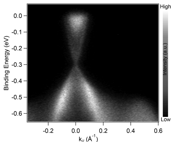
FIG. 4. ARPES intensity image of \text{Fe}_{0.2}\text{Bi}_2\text{Se}_3 taken at T = 10 K along the \bar{\Gamma} - \bar{M} direction with photons of 21.2 eV.
