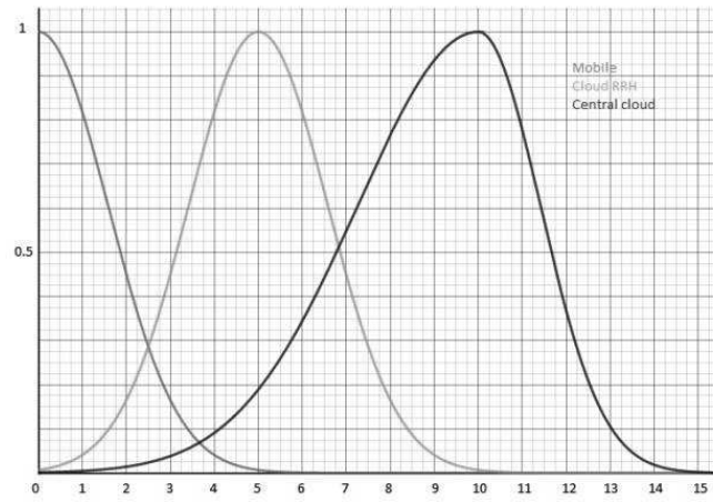
Figure 4: Membership functions
