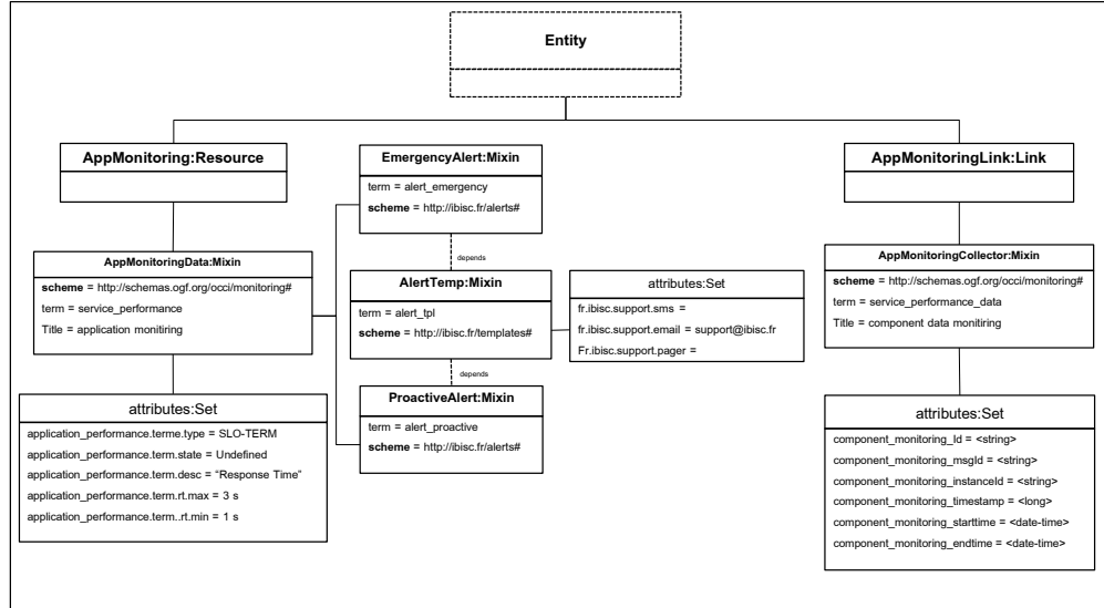
Fig. 2: Monitoring OCCI Model
