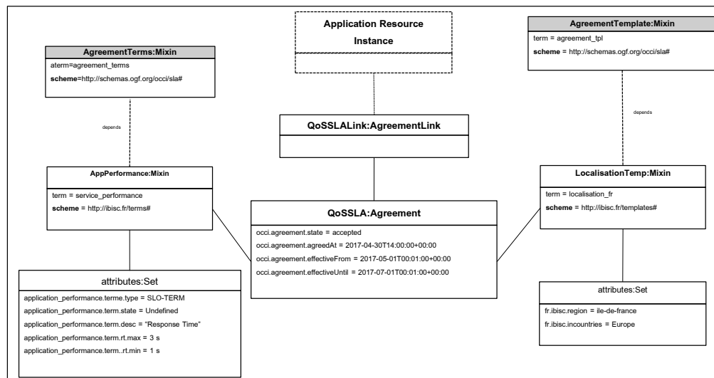
Fig. 1: Application OCCI SLA Model
