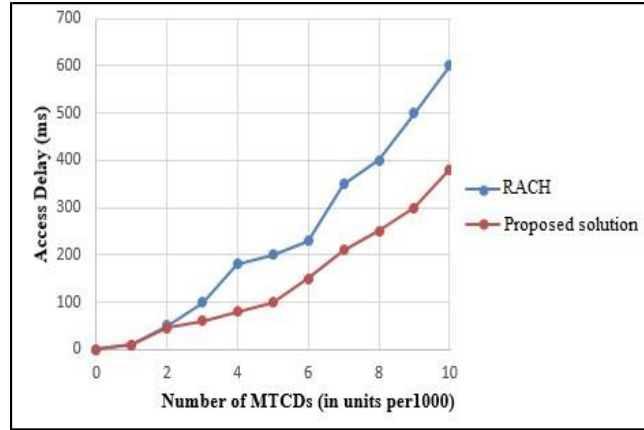
Figure 7: Access Delay
