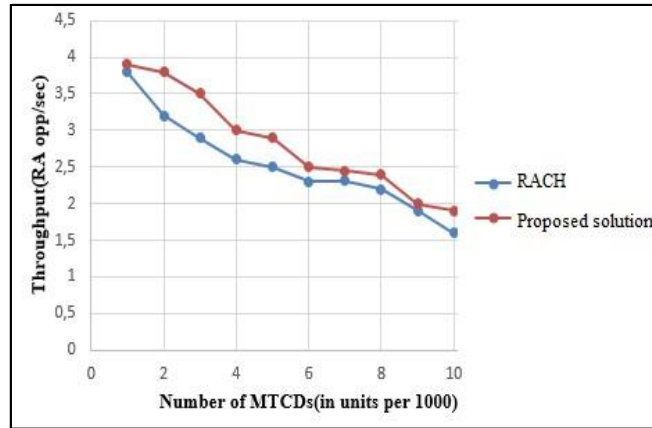
Figure 6: Throughput
