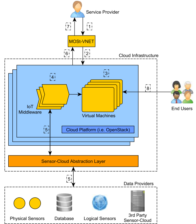
Figure 2. MOST-VNET in a Cloud Computing and Internet of Things context.
