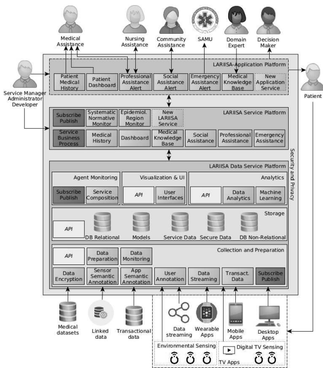
Figure 4. LARIISA architecture
