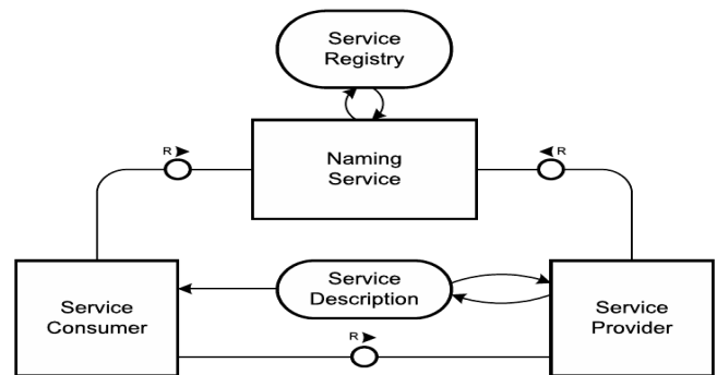
Figure 3. A typical Service-Oriented Architecture [8]
