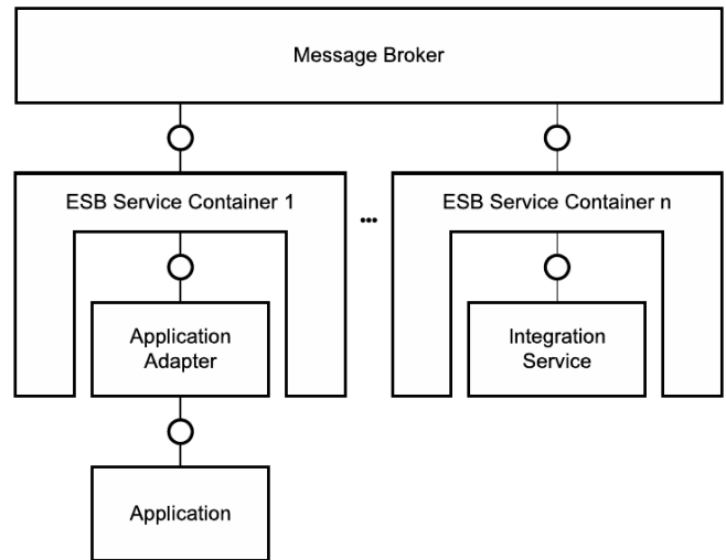
Figure 5. A simple ESB scenario [8]
