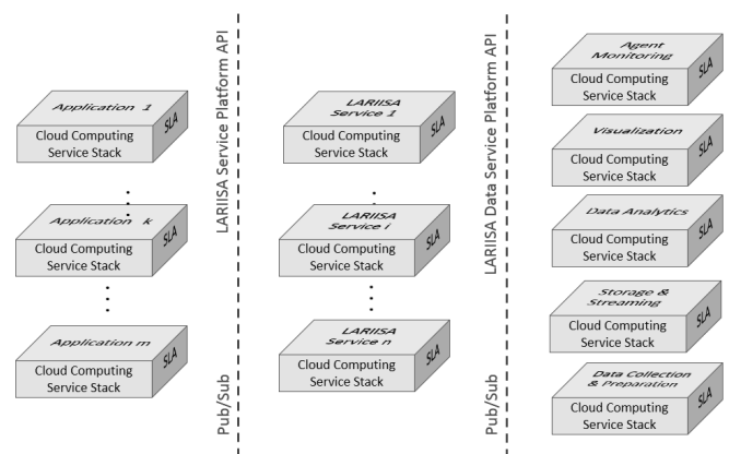
Figure 7. An illustration of service composition of LARIISA framework prior to cloud deployment
