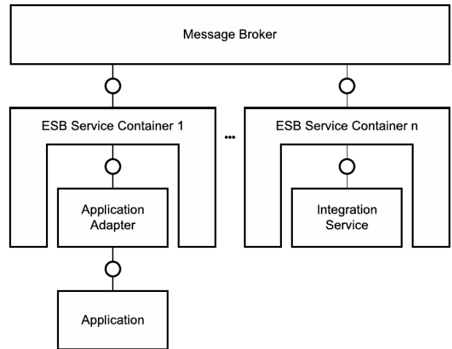
Figure 5. A simple ESB scenario [8]
